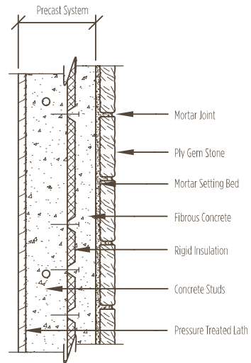
Stone Over S.W. Precast Walls
