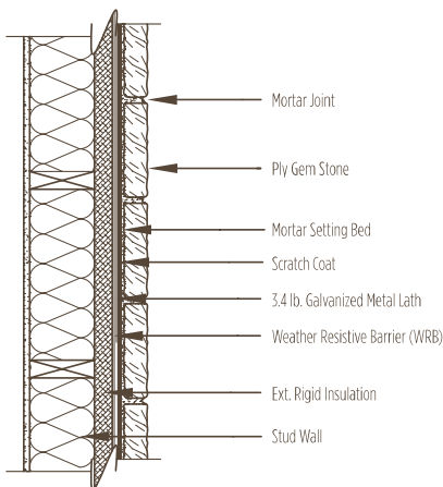
Stone Over Rigid Insulation Wall
